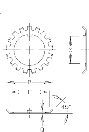
Figure 2 – Lockwashers
