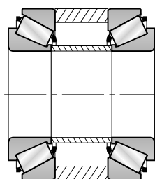
IsoClass Spacer Assemblies
