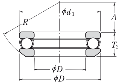
With Aligning Seat
