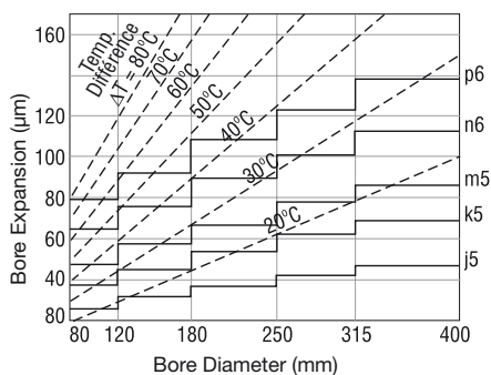
Figure 1 – Temperature and Expansion of Inner Ring
