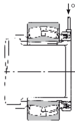
Removal Using a Hydraulic Nut
