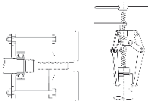
Removal of Inner Ring with Withdrawal Tools
