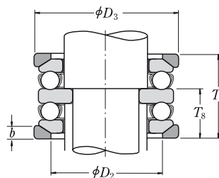
With Aligning Seat Washer
