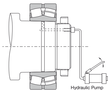
Removal Using Oil Injection
