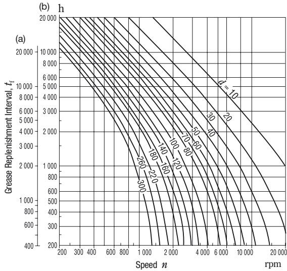
(1) Radial Ball Bearings (a), Cylindrical Roller Bearings (b)
