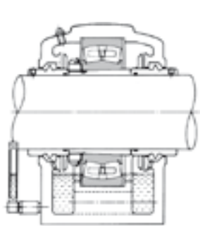
Oil Bath Lubrication: not for high speeds
