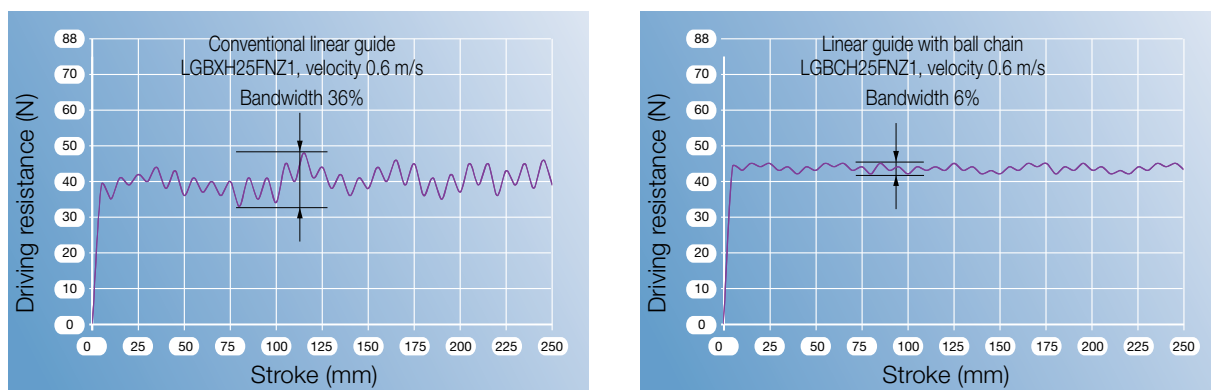
Figure 1.11 Driving resistance
