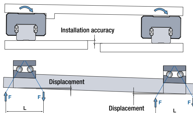
Figure 1.5 Internal forces for DF- and DB-configuration
