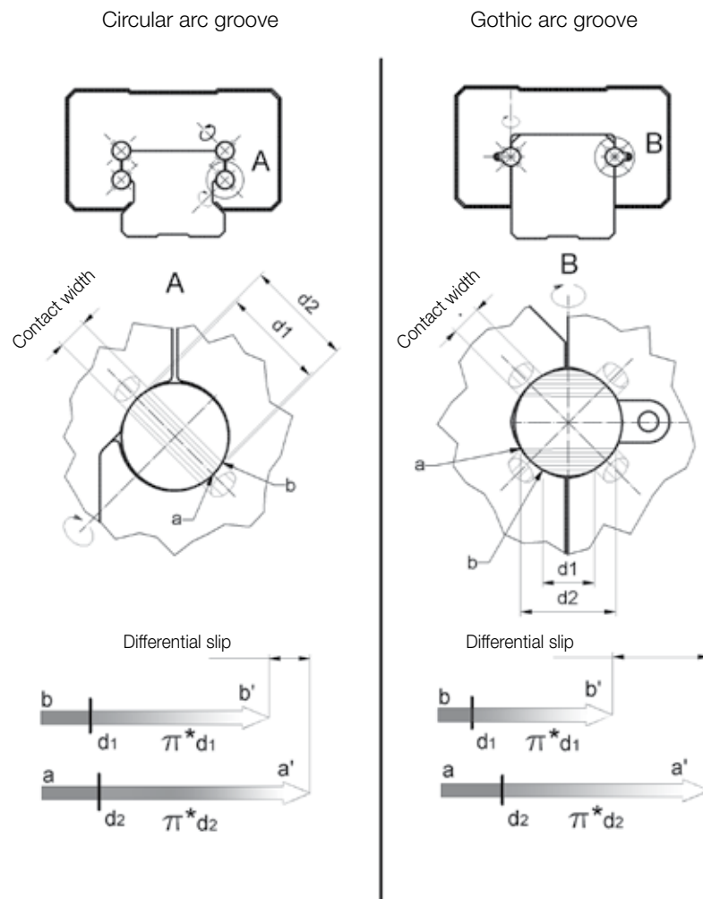
Figure 1.3 Groove geometry
