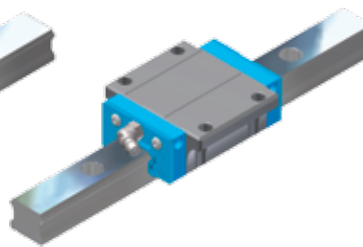
LGBXS...FN (standard)
