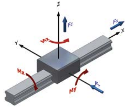
Figure 2.1 Coordinate system
