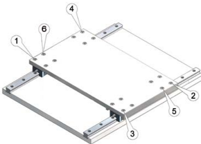
Figure 3.14 Fastening sequence for machine table installation
