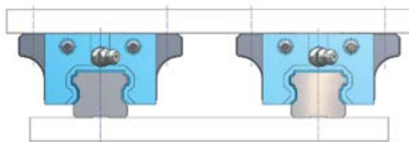
Two-rail arrangement (2)
