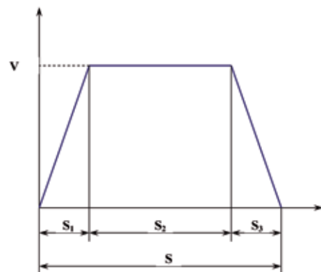
Figure 2.16 Velocity/distance diagram
