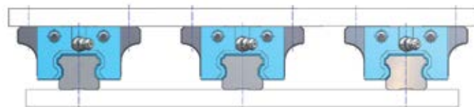
Three-rail arrangement (3)
