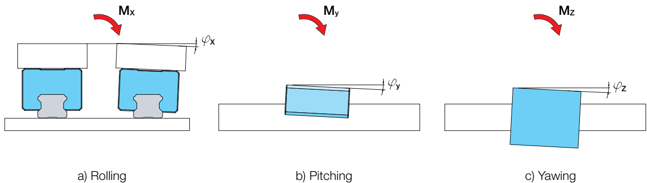
Figure 2.19 Angular deformation due to torque load
