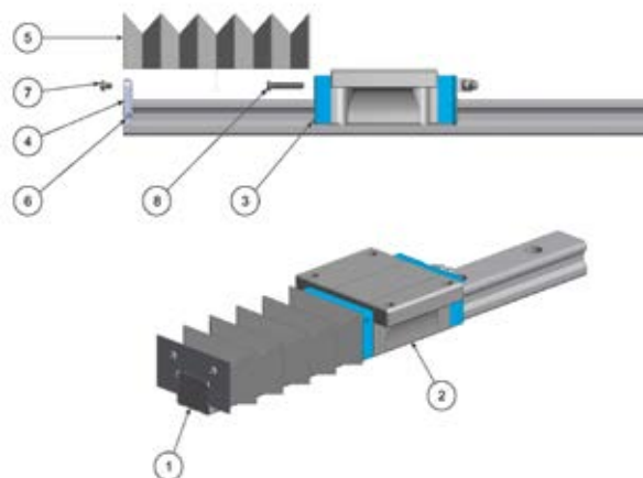
Figure 5.4 Assembly of bellows
