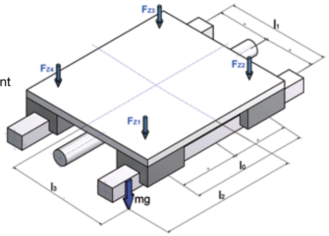
Figure 2.12 Calculation example 2
