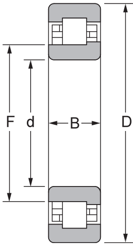
NJ
