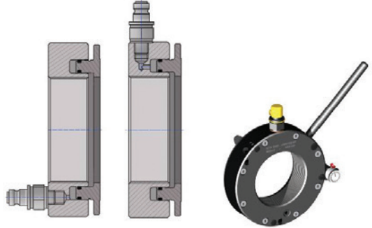
Optional connection at: Face side or Outer shell
