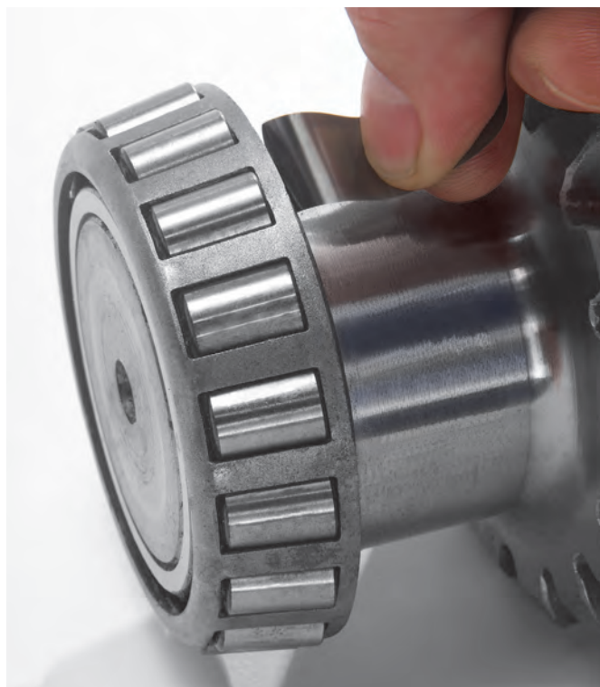
Fig. 23. Bearings should be checked with a feeler gage to ensure proper fit.
