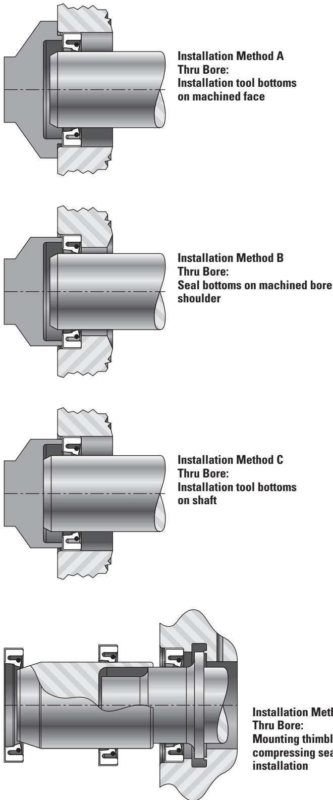
Fig. 61. Installation methods.
