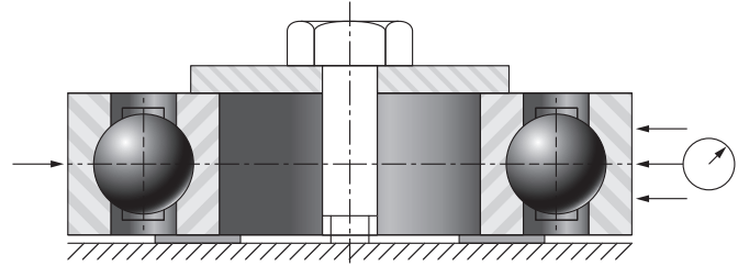
Fig. 12. RIC can be measured mechanically by moving the outer ring horizontally.
